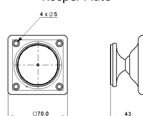
Keeper Plate
