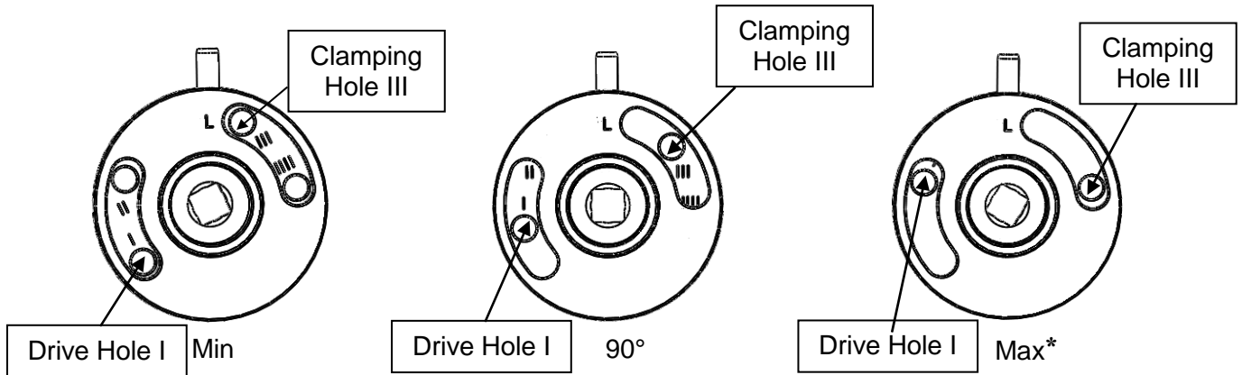
Figure 3: Left Hand Parallel Arm Cam Positions
