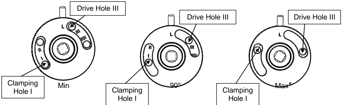
Figure 1: Left Hand Projecting Arm Cam Positions
