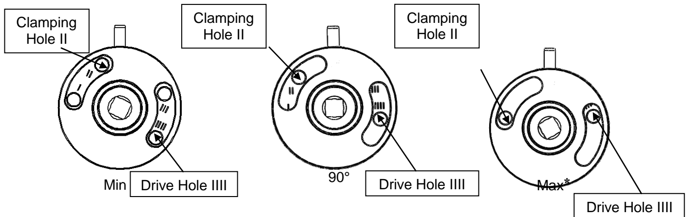
Figure 4: Right Hand Parallel Arm Cam Positions
