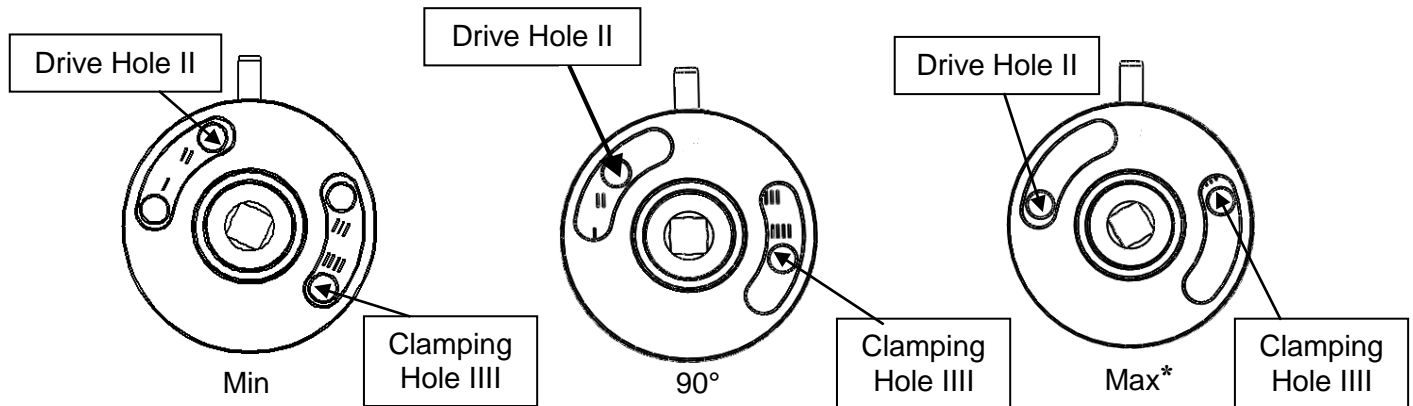
Figure 2: Right Hand Projecting Arm Cam Positions
