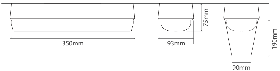
Image shows from left to right show side profile and end views of standard fitting and with drop down legend
